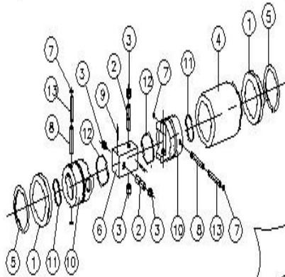
UNIVERSAL JOINT DETAIL ASSEMBLY
